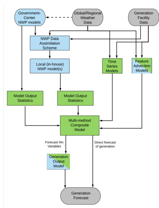
Figure 1: High-level overview of the components and data flow of a typical state-of-the-art forecasting solution.
